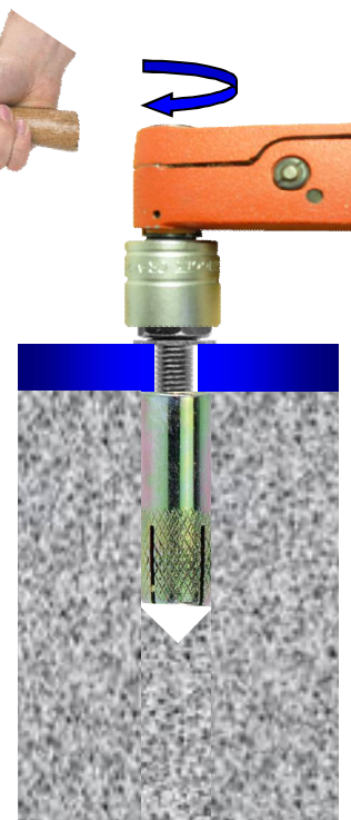
Tighten with torque wrench to recommended torque
